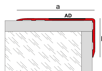
Novopeldaño® Safety
